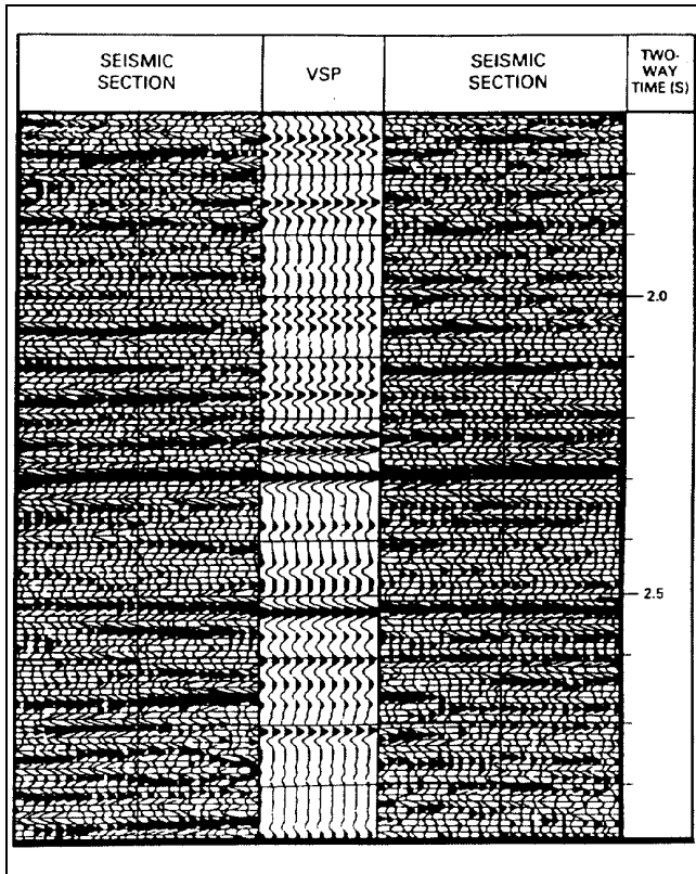
Figure 7-51. Example of correlation between VSP and surface seismic profiling; the VSP data stack is shown at the proper well location with respect to the seismic section
