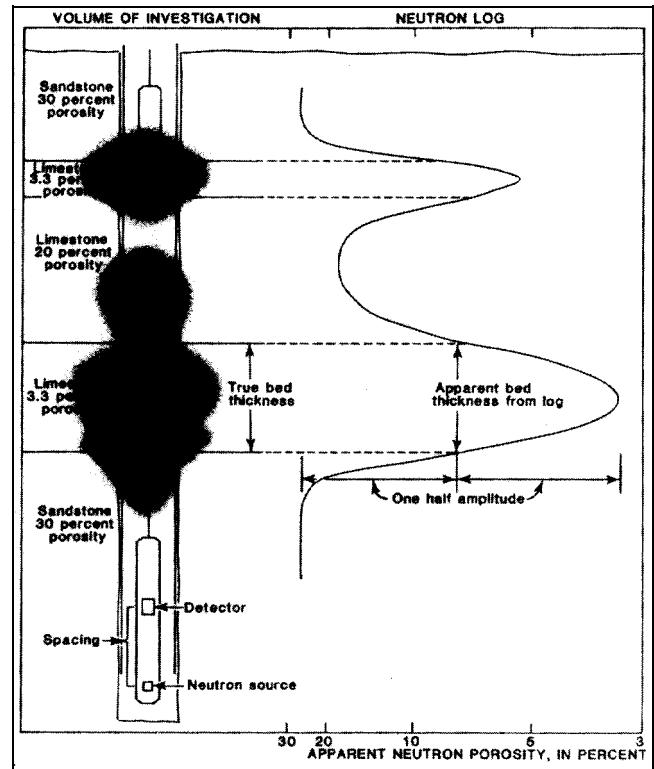
Figure 7-20. Theoretical response of a neutron probe to changes in porosity and bed thickness. The shaded area represents the volume of investigation at different probe positions
