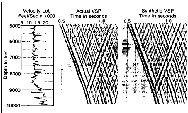
Figure 7-60. Comparison of real and synthetic VSP's
