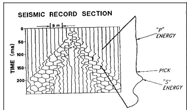
Figure 3-27. Example of shear-wave record. Expanded trace identifies "S" and "P" energy confirmed by dual trace plots
