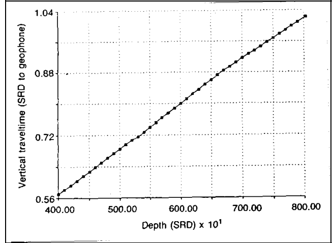
Figure 7-55. Vertical time-depth plot corrected to SRD
