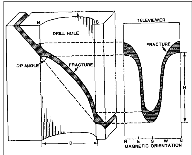
Figure 7-30. Three-dimensional view of a fracture and appearance of the same fracture on an acoustic-televiwer log. D is borehole diameter and h is the length of the fracture intercept in the borehole
