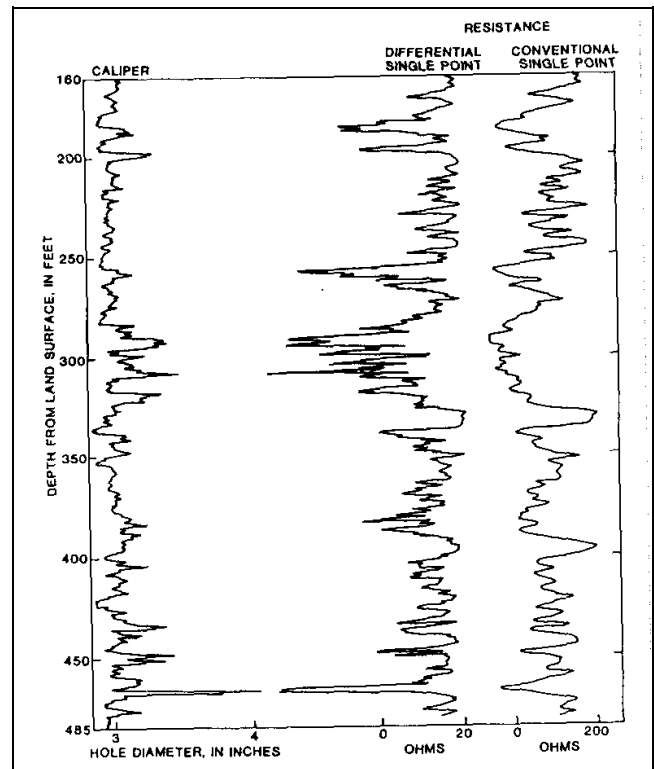
Figure 7-9. Caliper, differential, and conventional single-point resistance logs in a well in fractured crystalline rocks
