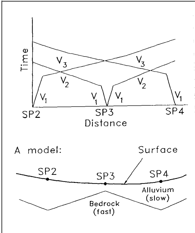
Figure 3-23. Cross-channel travel-time schematic
