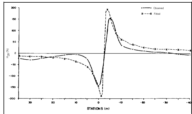
Figure 4-61. VLF profile over buried telephone line (Wright 1988; copyright permission granted by Scintrex)
