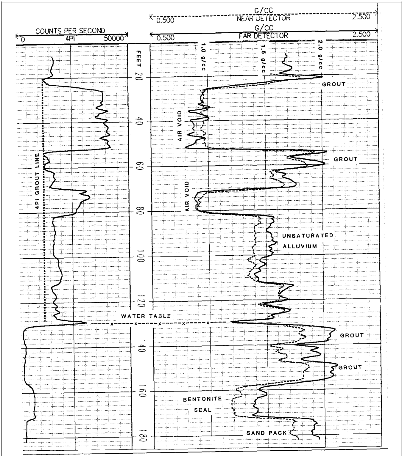
Figure 7-43. Dual-spaced and "4π" density logs in a cased monitoring well showing completion as interpreted from the logs (Yearsley, Crowder, and Irons 1991; copyright permission granted by Colog, Inc.)
