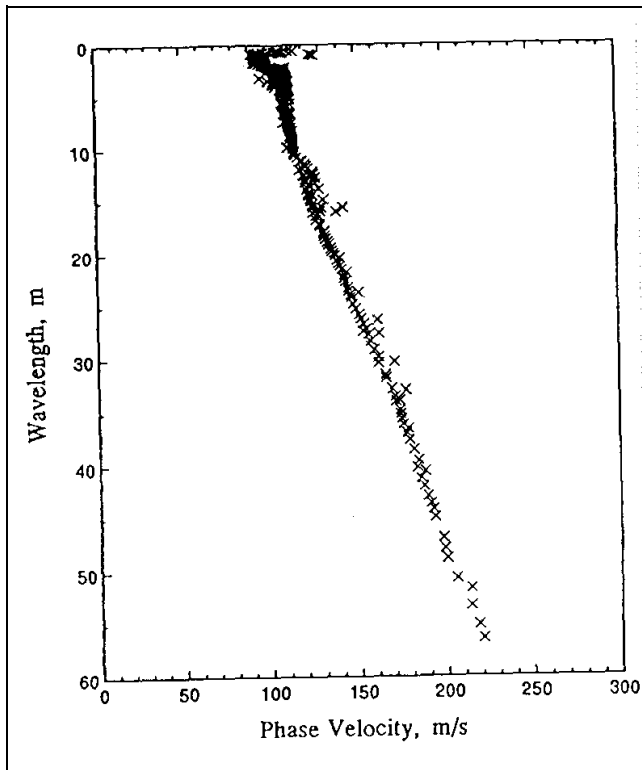
Figure 3-35. Typical SASW data
