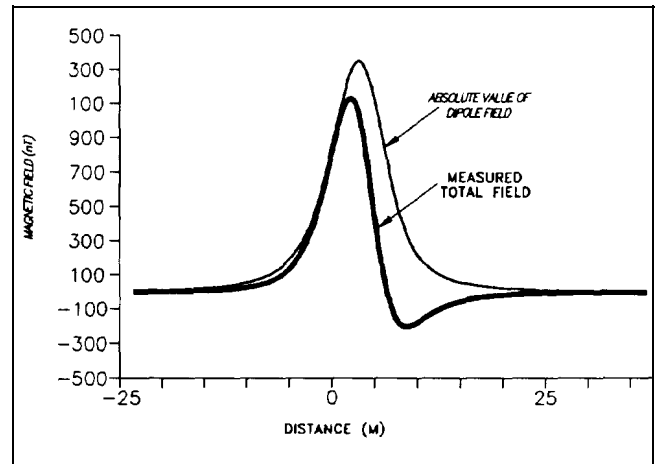
Figure 6-2. Actual and measured fields due to magnetic inclination
