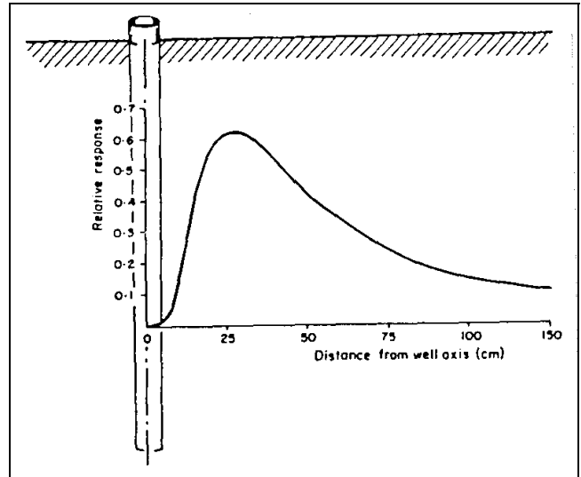
Figure 7-17. Relative response of an induction probe with radial distance from borehole axis (copyright permission granted by Geonics Limited)
