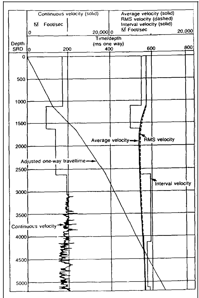
Figure 7-56. Example of final display from velocity survey shown with sonic log
