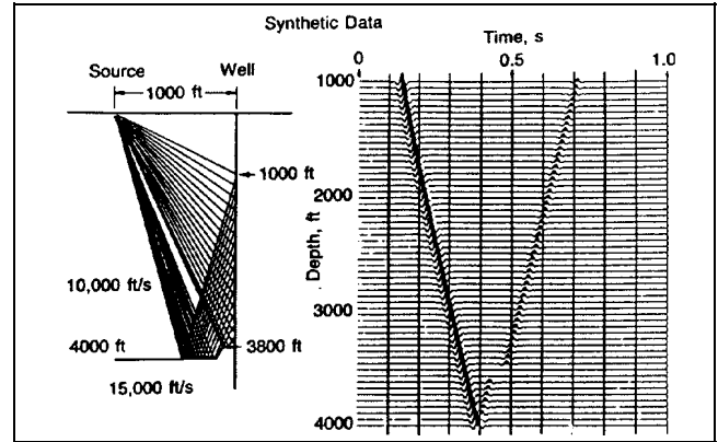
Figure 7-52. Model of fault structure
